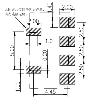
RECOMMENDED PCB LAYOUT TOP VIEW (. XX ± 0.05)
