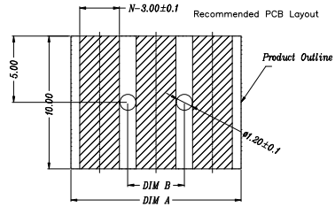
RECOMMENDED PCB LAYOUT TOL:(±0.05)
