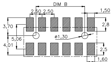
RECOMMENDED PCB LAYOUT TOP VIEW (. XX ± 0.05)
