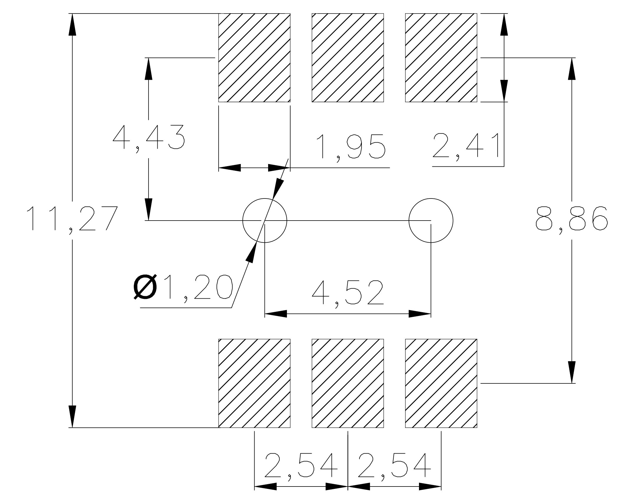
RECOMMENDED PCB LAYOUT TOP VIEW (. XX ± 0.05)
