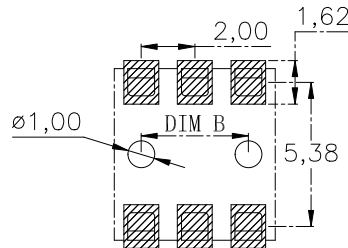
RECOMMENDED PCB LAYOUT TOP VIEW (. XX ± 0.05)
