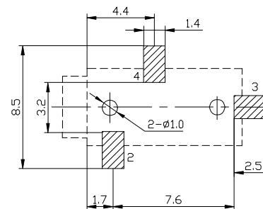
HOLE LAYOUT
