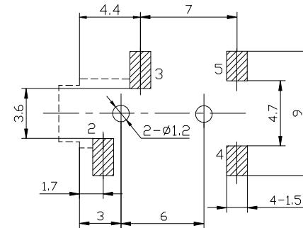
HOLE LAYOUT
