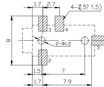
HOLE LAYOUT
