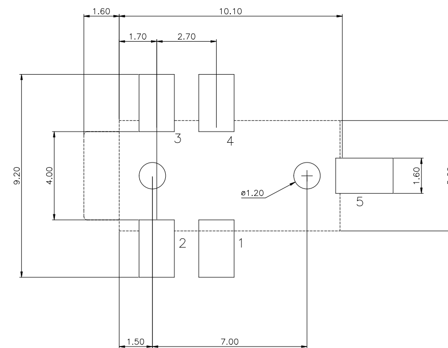
HOLE LAYOUT
