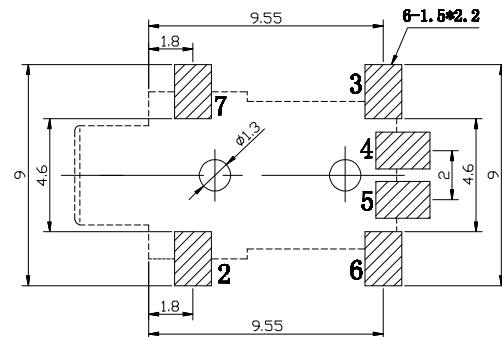
HOLE LAYOUT
