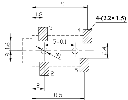
HOLE LAYOUT
