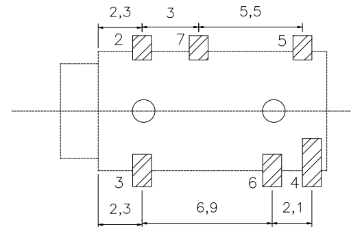
HOLE LAYOUT
