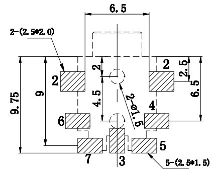
HOLE LAYOUT
