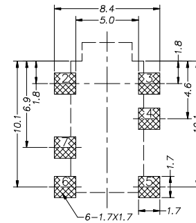
HOLE LAYOUT
