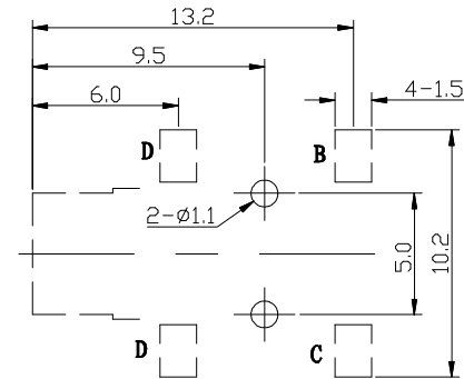
HOLE LAYOUT
