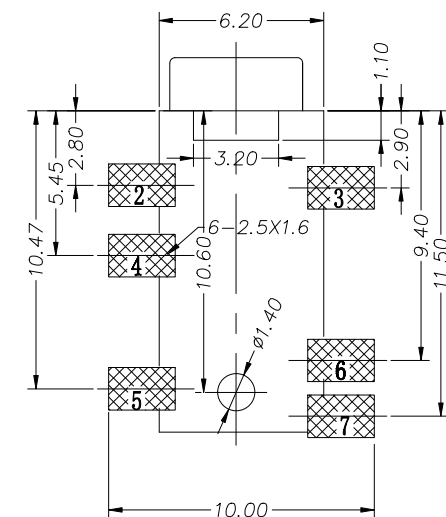
HOLE LAYOUT
