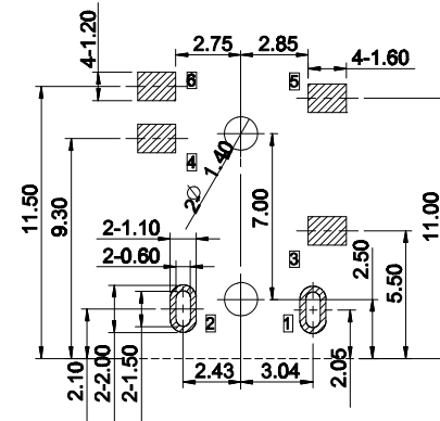
HOLE LAYOUT
