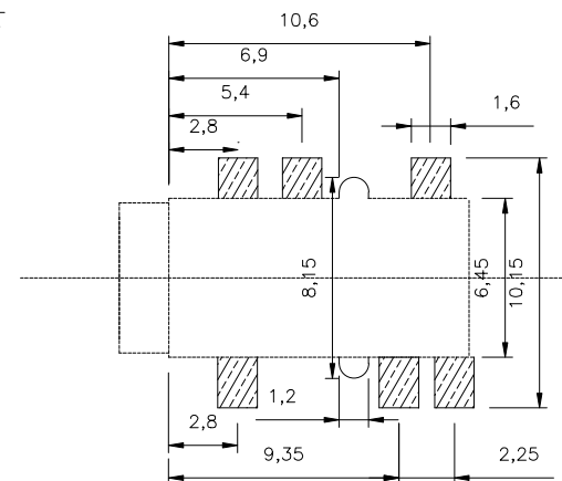
HOLE LAYOUT
