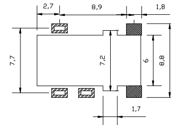
HOLE LAYOUT
