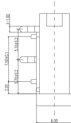
SCHEMATIC
