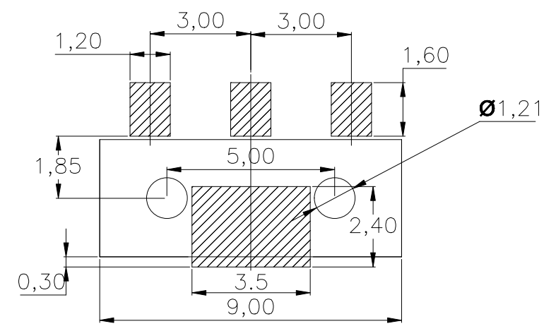
RECOMMENDED PCB LAYOUT TOL:(±0.05)
