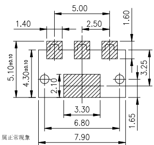
RECOMMENDED PCB LAYOUT TOP VIEW (. XX ± 0. 05)
