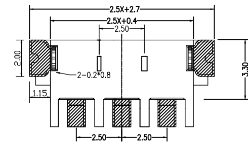
PCB LAYOUT (3pin)
