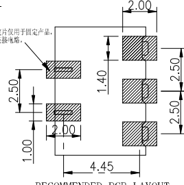
RECOMMENDED PCB LAYOUT TOP VIEW (. XX ± 0. 05)
