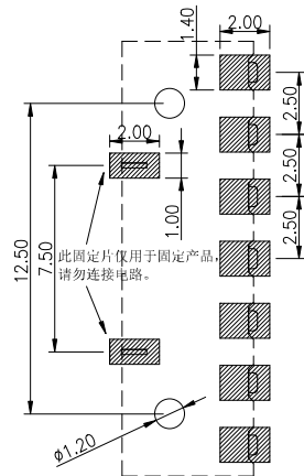
RECOMMENDED PCB LAYOUT TOP VIEW (XX±0.05)
