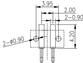
RECOMMENDED P.C.B LAYOUT TOP VIEW (.XX±0.05)
