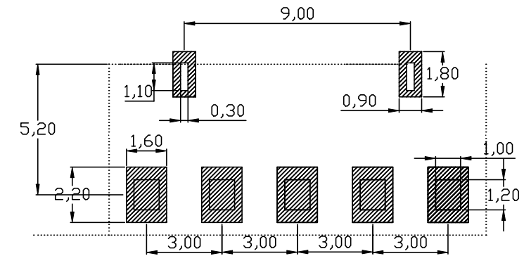
RECOMMENDED PCB LAYOUT TOP VIEW (.XX±0.05)
