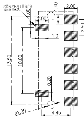
RECOMMENDED PCB LAYOUT TOP VIEW (. XX ± 0. 05)
